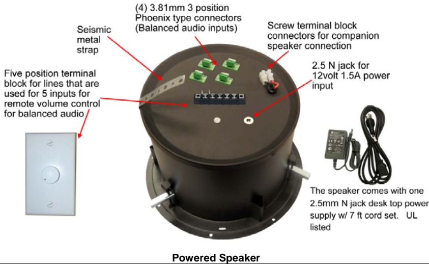
Powered Speaker
