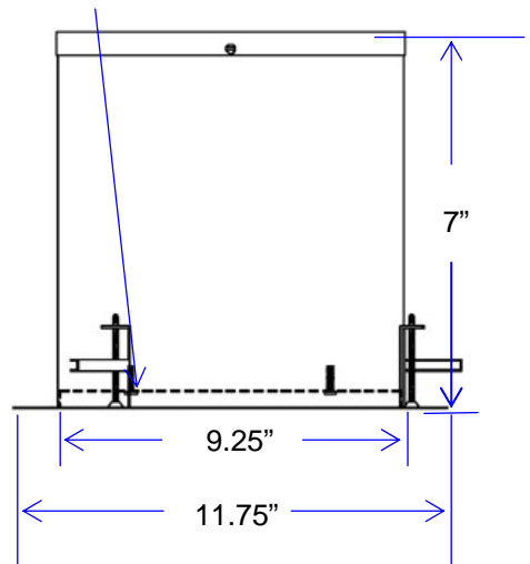
Recessed speaker baffle plate
