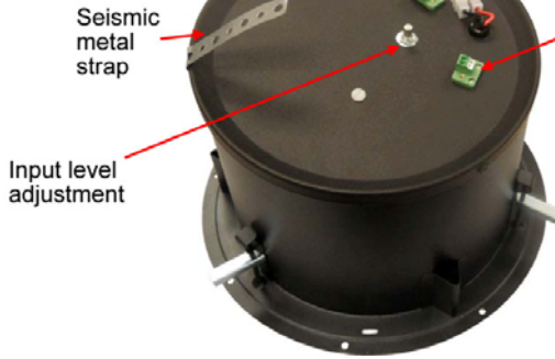
Powered Speaker
