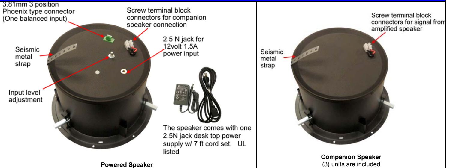
Powered Speaker
