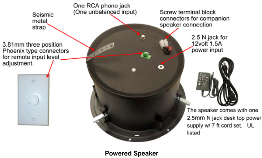
Powered Speaker
