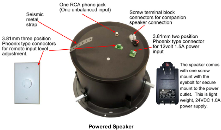
Powered Speaker
