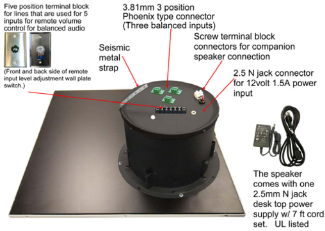
Powered Speaker
