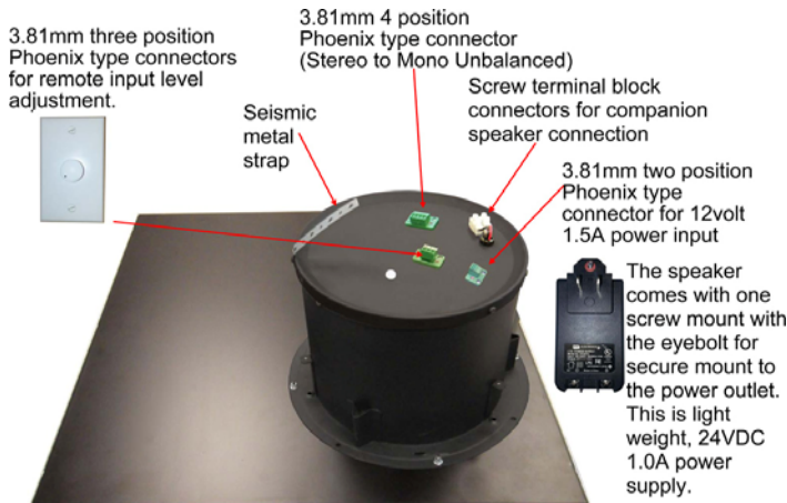
Powered Speaker
