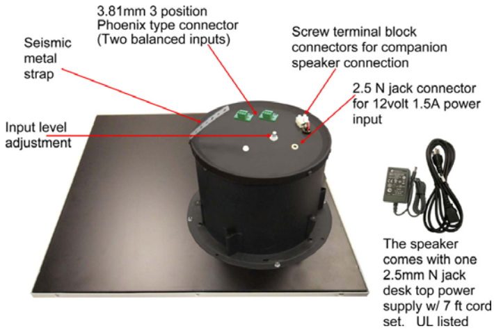
Powered Speaker
