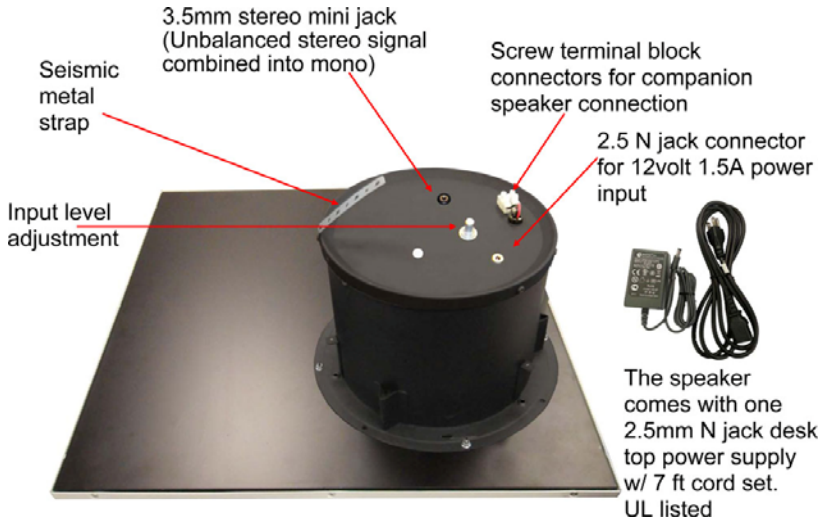
Powered Speaker
