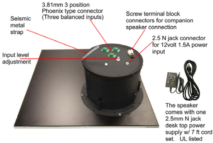
Powered Speaker
