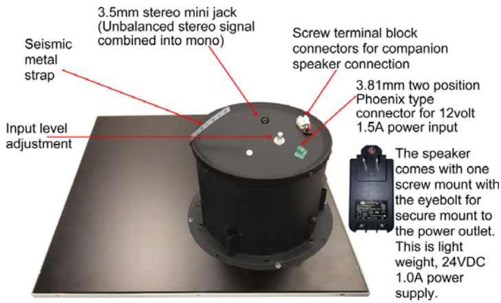
Powered Speaker
