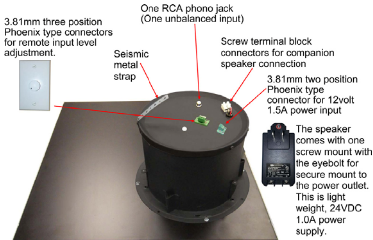
Powered Speaker
