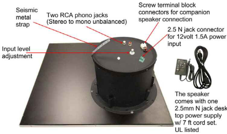
Powered Speaker
